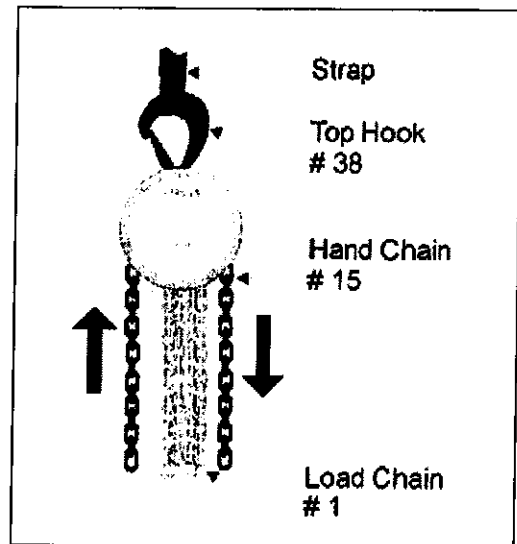
Figure 2- Raising the Load
