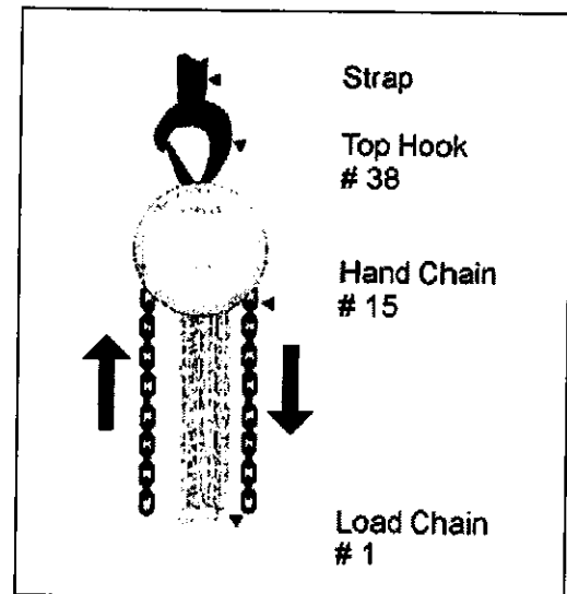
Figure 3- Lowering the Load
